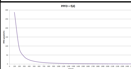
Photosynthetic Photon Flux Density (PPFD) as a function of distance from single TINY RH
