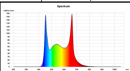
SKYLIGHT TINY RH spectrum
